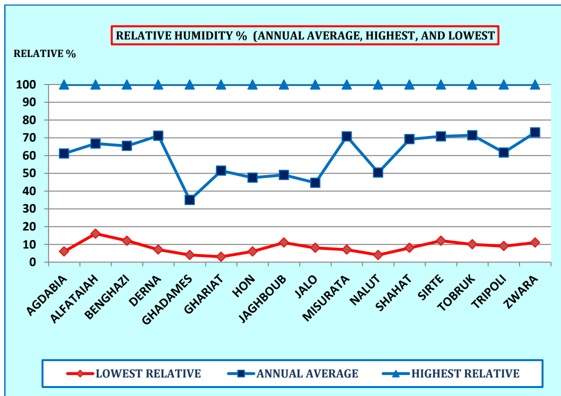
Figure 18. Average Relative Humidity (%) for Annual, Highest, Lowest (1971-2010)
