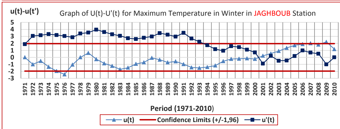
Figure 137. Graphs of M-K U(t)-U'(t) Results for Maximum Temperature in Winter in GHADAMES, GHARIAT, HON and JAGHBOUB Stations
