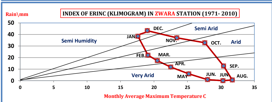
Figure 39. Index of Erinç (Klimograms) in SIRTE, TOBRUK, TRIPOLI and ZWARA stations (1971-2010)
