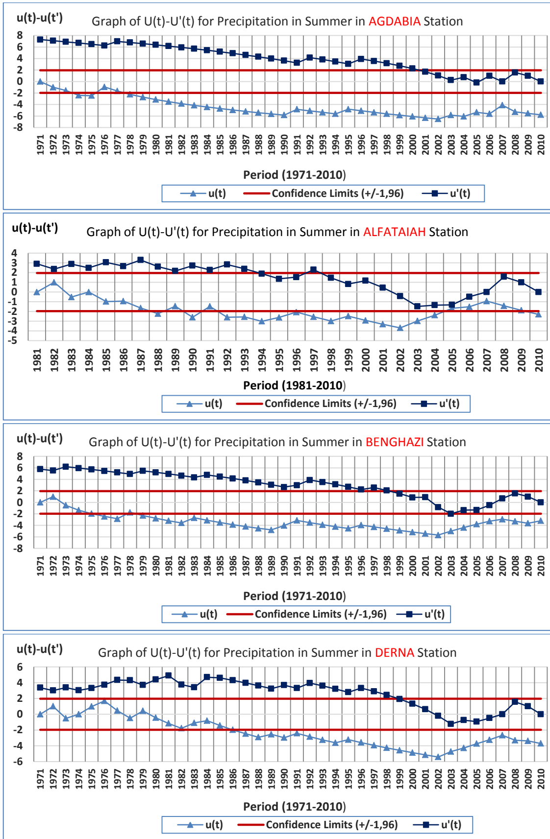
Figure 244. Graphs of M-K U(t)-U'(t) Results for Precipitation in Summer in AGDABIA, ALFATAIAH, BENGHAZI and DERNA Stations
