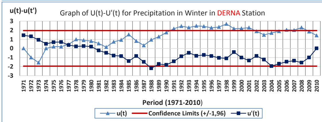
Figure 252. Graphs of M-K U(t)-U'(t) Results for Precipitation in Winter in AGDABIA, ALFATAIAH, BENGHAZI and DERNA Stations
