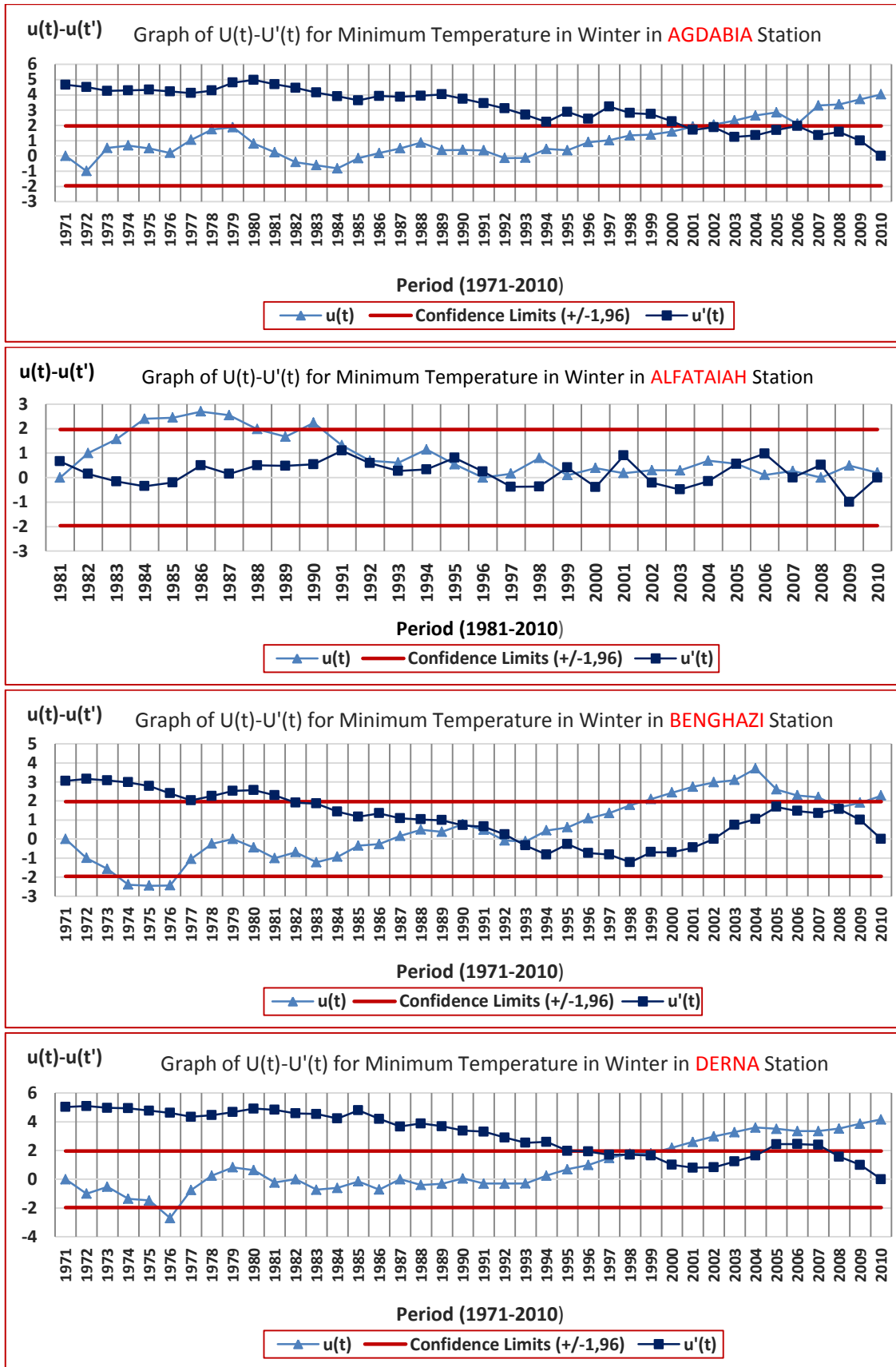
Figure 156. Graphs of M-K U(t)-U'(t) Results for Minimum Temperature in Winter in AGDABIA, ALFATAIAH, BENGHAZI and DERNA Stations
