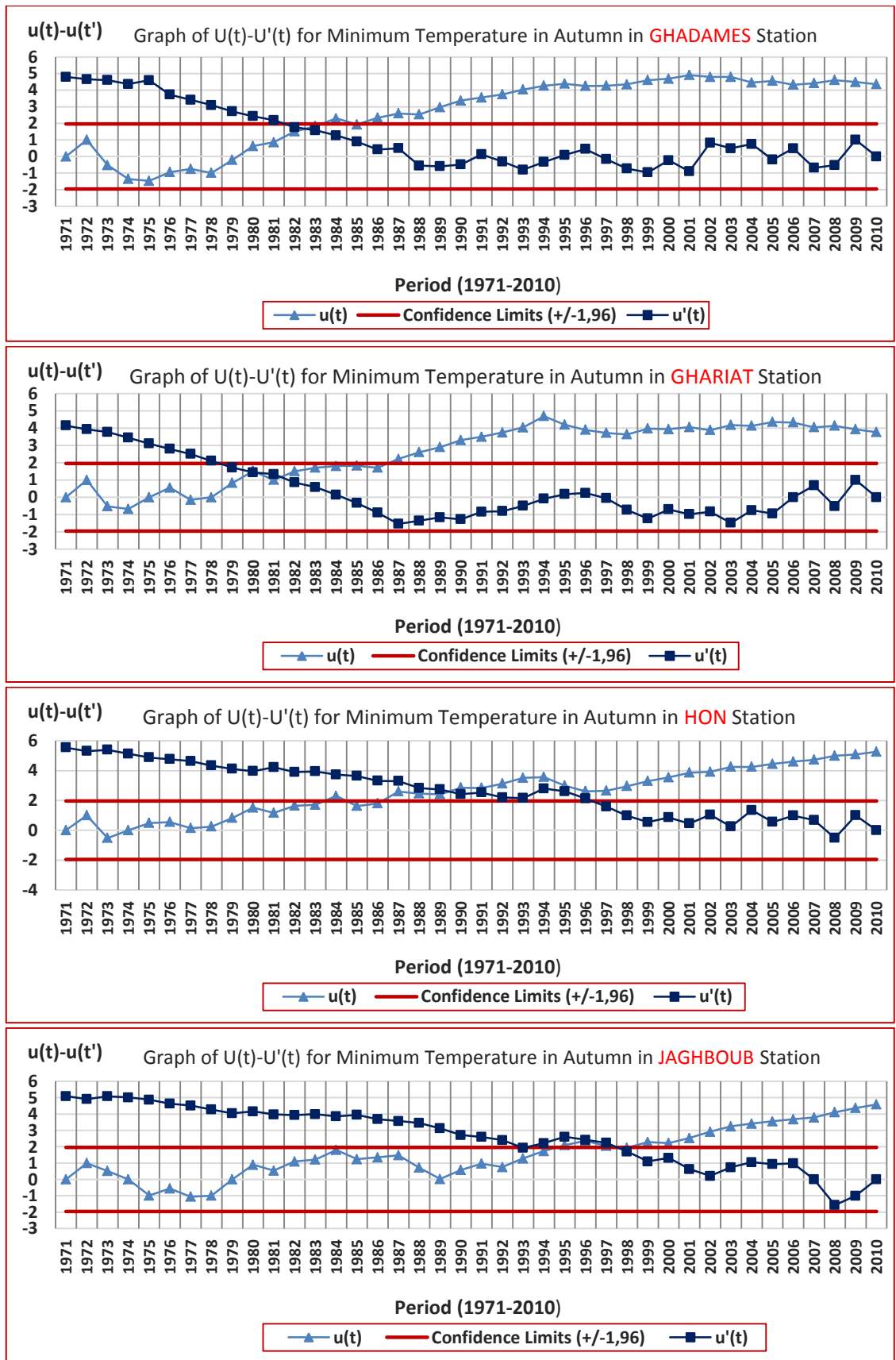
Figure 153. Graphs of M-K U(t)-U'(t) Results for Minimum Temperature in Autumn in GHADAMES, GHARIAT, HON and JAGHBOUB Stations
