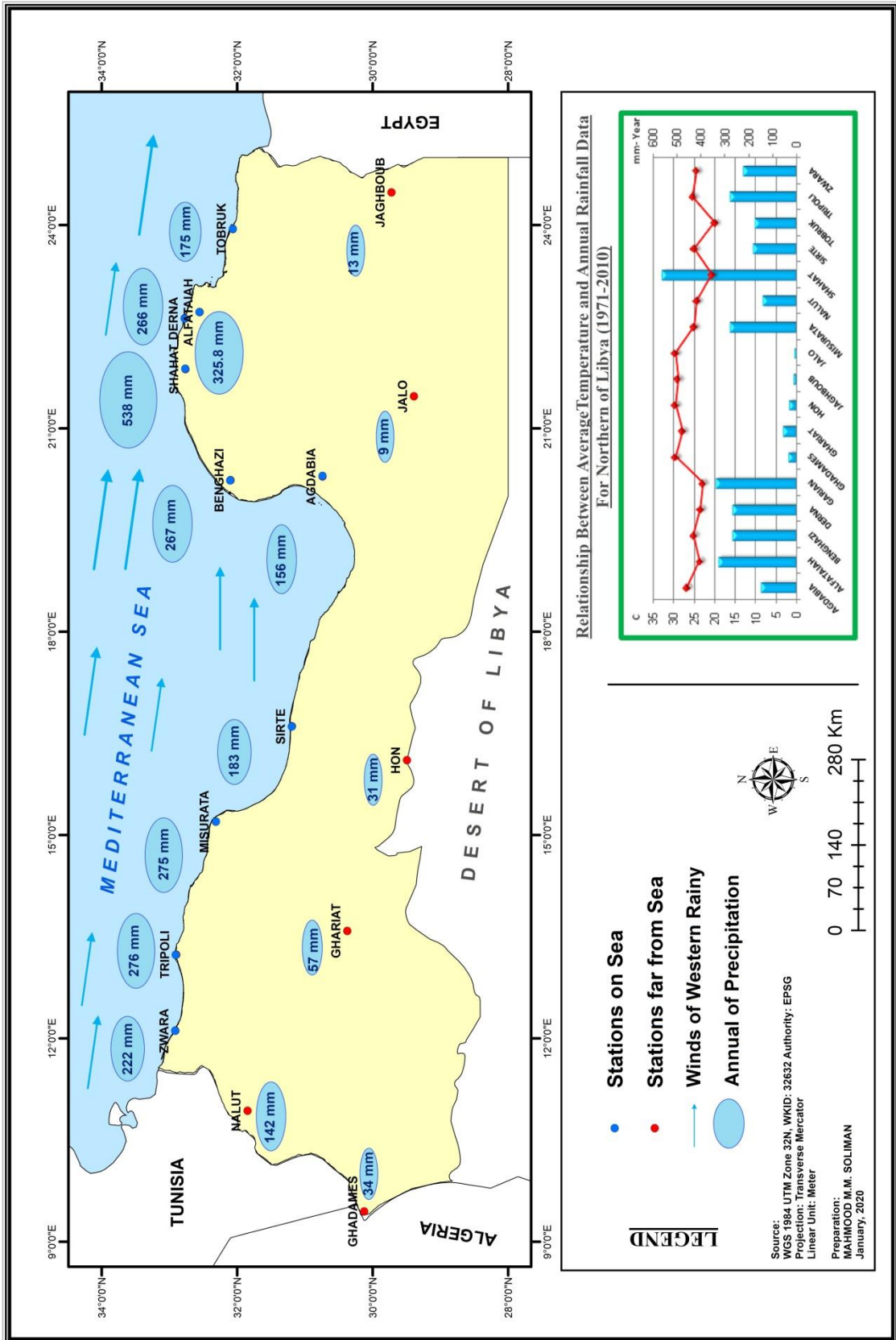
Map 7. The Relationship Between Direction of Coastline and Precipitation
