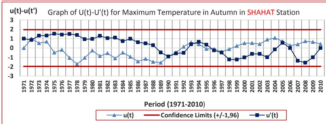
Figure 134. Graphs of M-K U(t)-U'(t) Results for Maximum Temperature in Autumn in JALO, MISURATA, NALUT and SHAHAT Stations
