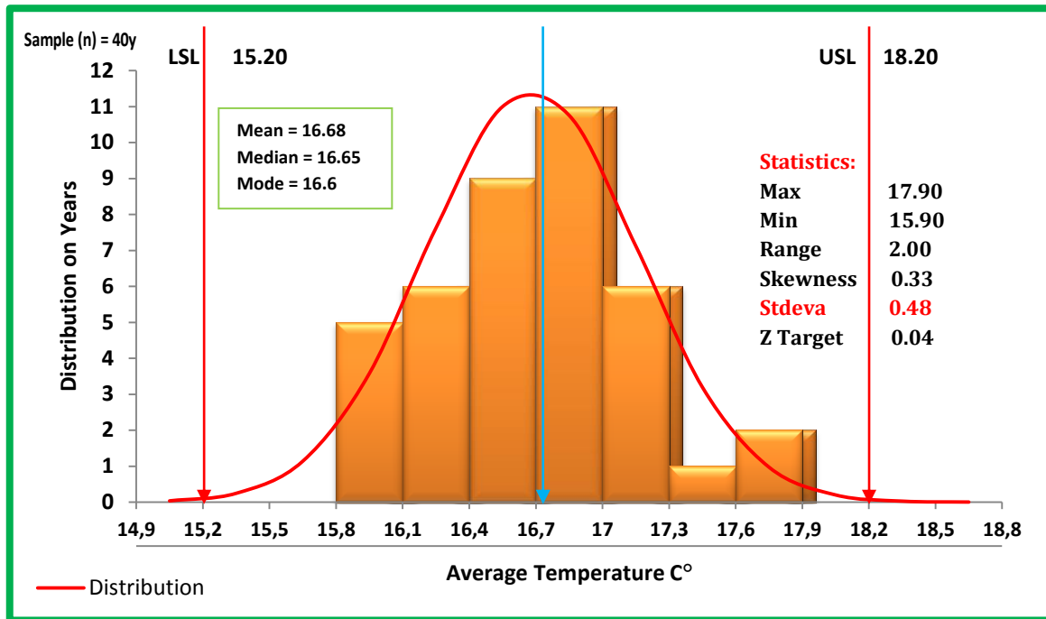
Figure 79. Statistics of Annual Average Temperature in SHAHAT Station for Period (1971-2010)
