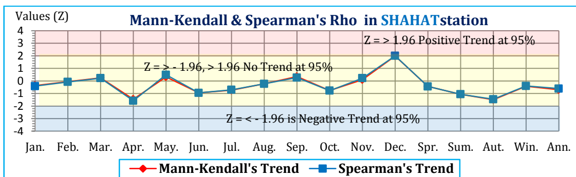
Figure 237. Mann-Kendall And Spearman's Trend for Precipitation in NALUTI and SHAHAT Stations (1971-2010)
