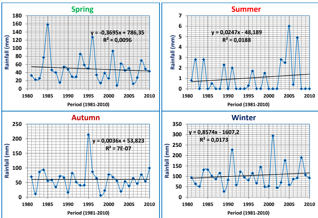
Figure 261. Simple Linear Trend Graphs of Seasonally Precipitation in ALFATAIAH Station (1981-2010)
