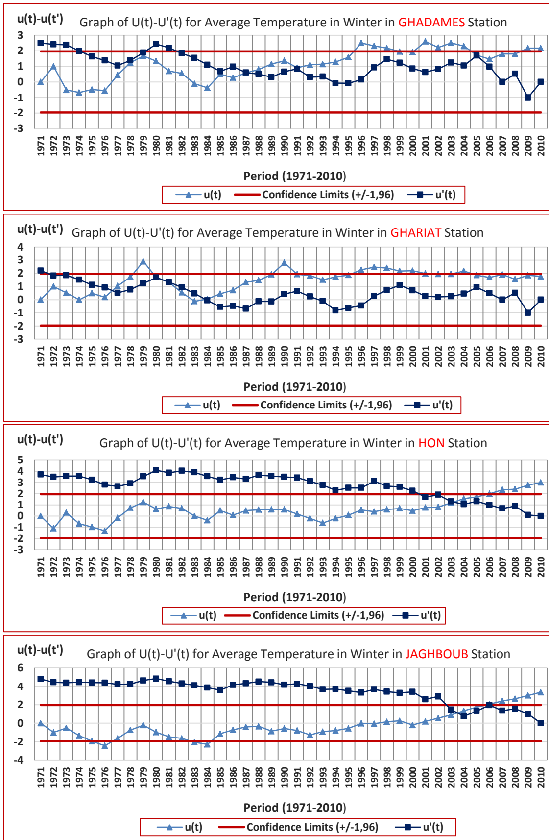
Figure 177. Graphs of M-K U(t)-U'(t) Results for Average Temperature in Winter in GHADAMES, GHARIAT, HON and JAGHBOUB Stations
