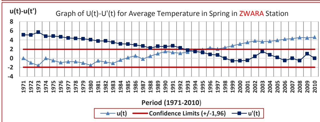
Figure 167. Graphs of M-K U(t)-U'(t) Results for Average Temperature in Spring in SIRTE, TOBRUK, TRIPOLI and ZWARA Stations
