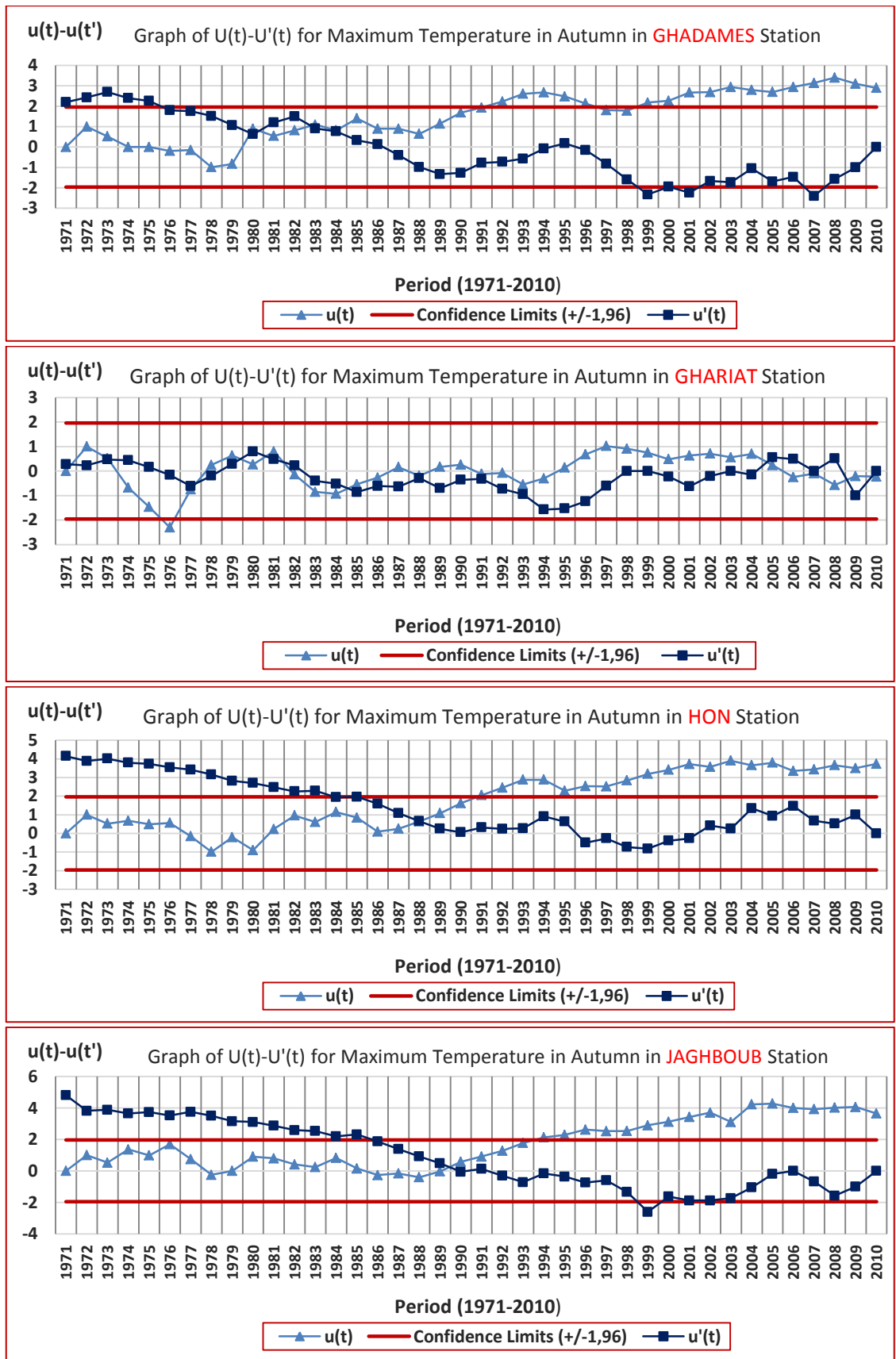
Figure 133. Graphs of M-K U(t)-U'(t) Results for Maximum Temperature in Autumn in GHADAMES, GHARIAT, HON and JAGHBOUB Stations
