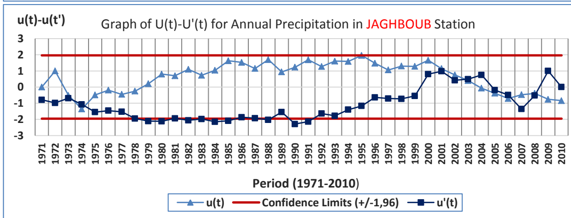
Figure 257. Graphs of M-K U(t)-U'(t) Results for Annual Precipitation in GHADAMES, GHARIAT, HON and JAGHBOUB Stations
