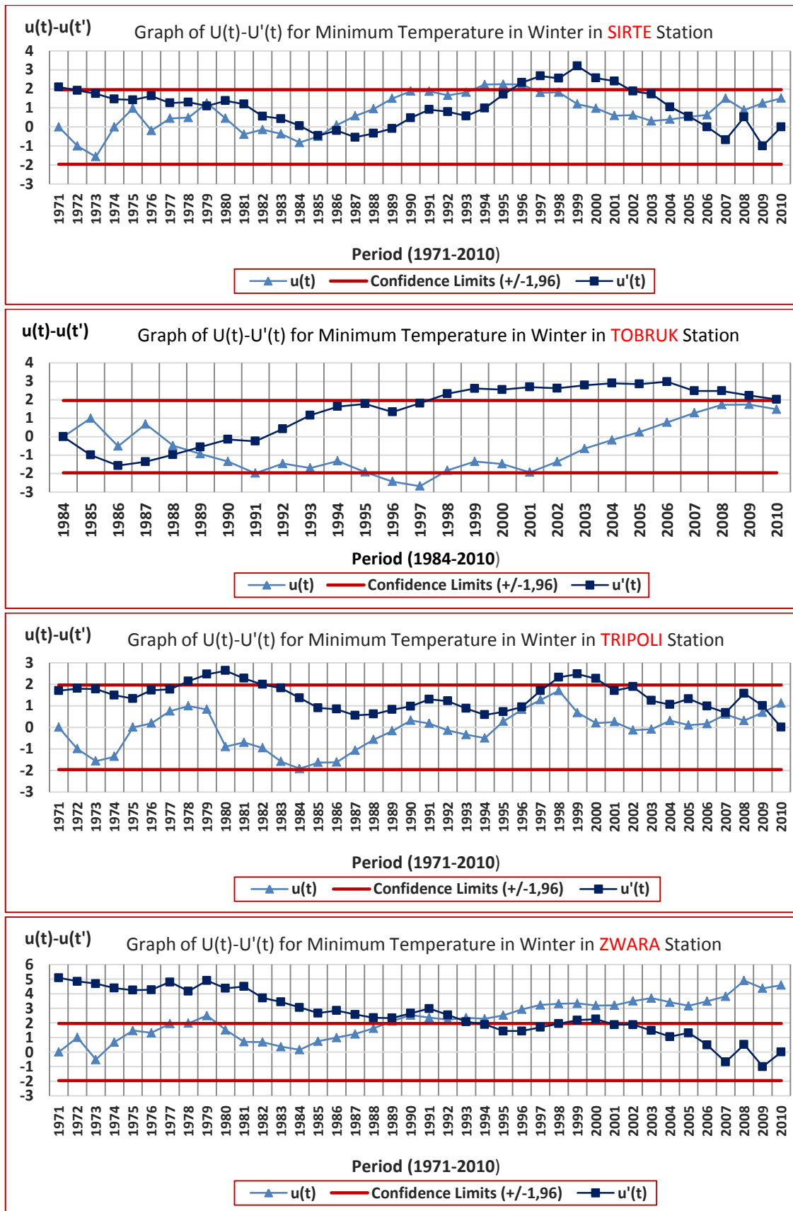
Figure 159. Graphs of M-K U(t)-U'(t) Results for Minimum Temperature in Winter in SIRTE, TOBRUK, TRIPOLI and ZWARA Stations
