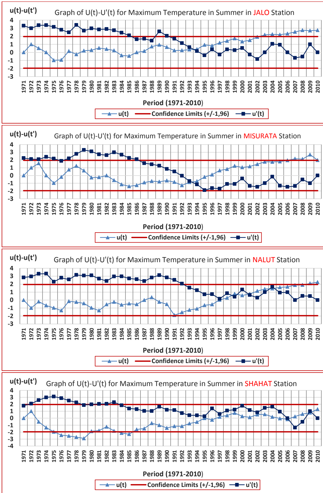
Figure 130. Graphs of M-K U(t)-U'(t) Results for Maximum Temperature in Summer in JALO, MISURATA, NALUT and SHAHAT Stations
