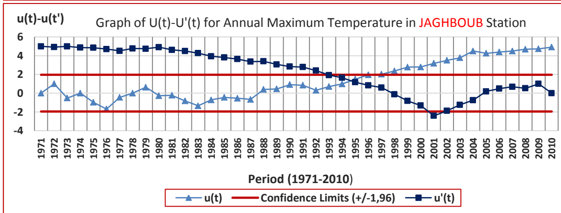
Figure 141. Graphs of M-K U(t)-U'(t) Results for Annual Maximum Temperature GHADAMES, GHARIAT, HON and JAGHBOUB Stations
