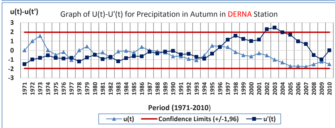
Figure 248. Graphs of M-K U(t)-U'(t) Results for Precipitation in Autumn in AGDABIA, ALFATAIAH, BENGHAZI and DERNA Stations
