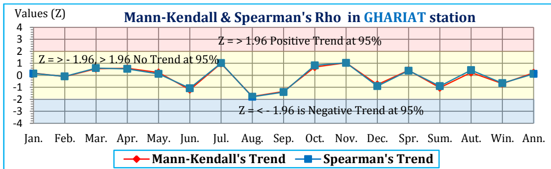
Figure 234. Mann-Kendall And Spearman's Trend for Precipitation in GHADAMES and GHARIAT Stations(1971-2010)
