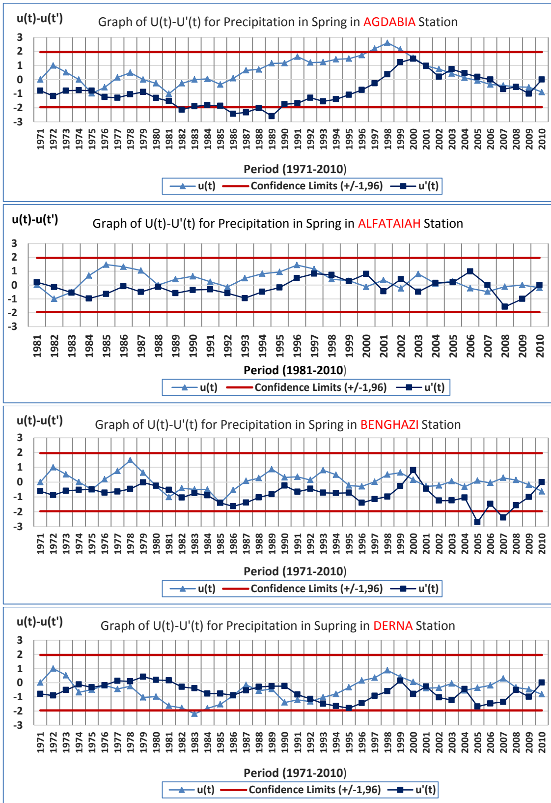
Figure 240. Graphs of M-K U(t)-U'(t) Results for Precipitation in Spring in AGDABIA, ALFATAIAH, BENGHAZI and DERNA Stations
