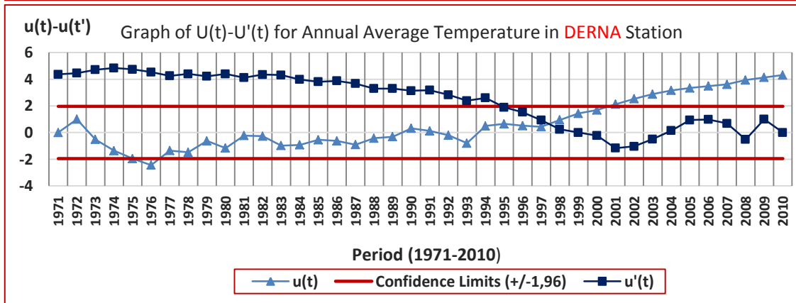
Figure 180. Graphs of M-K U(t)-U'(t) Results for Annual Average Temperature in AGDABIA, ALFATAIAH, BENGHAZI and DERNA Stations
